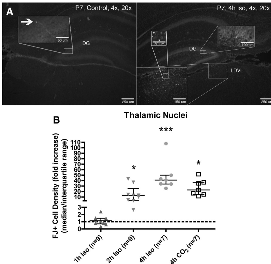
Fig. 3. Cell death in the thalamic nuclei. Example of FluoroJade-stained coronal brain sections from rats anesthetized with isoflurane (Iso) for 0 h (Control) and 4 h at postnatal day (P)7 (A). Unanesthetized rats had some naturally occurring cell death (arrow, for amount by area see table 1). Four-hour isoflurane significantly increased cell death in the thalamic nuclei (A, B) and mildly increased hippocampal cell death (A, also see Fig. 5A) as well as in other brain regions not shown here. For a detailed analysis of separate subregions, see table 1. Data are median fold increase from control group median (dotted line) with interquartile ranges. The raw cell death numbers in the control group can be found in table 1. * P < 0.05 , *** P < 0.001 , Kruskal-Wallis test with Dunn's correction for multiple comparisons. CO 2 = carbon dioxide; DG = dentate gyrus; LDVL = laterodorsal ventrolateral thalamic nucleus.
