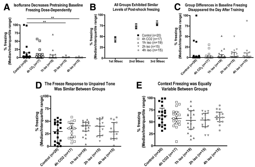
Fig. 6. Fear conditioning performance 8 weeks after 0-h, 1-h, 2-h, or 4-h isoflurane (iso) or 4-h carbon dioxide (CO 2 ) at post-natal day (P)7. Isoflurane given to P7 rats for 2 h or 4 h decreased baseline freezing (A) but not pretone test freezing (C). Tone-shock pairings resulted in short-term memory formation (B). There was a difference in neither the hippocampal-independent tone portion of the test (D) nor the hippocampal-dependent context portion (E). Data are medians with interquartile ranges. ** P < 0.01 , Kruskal-Wallis test with Dunn's correction.
